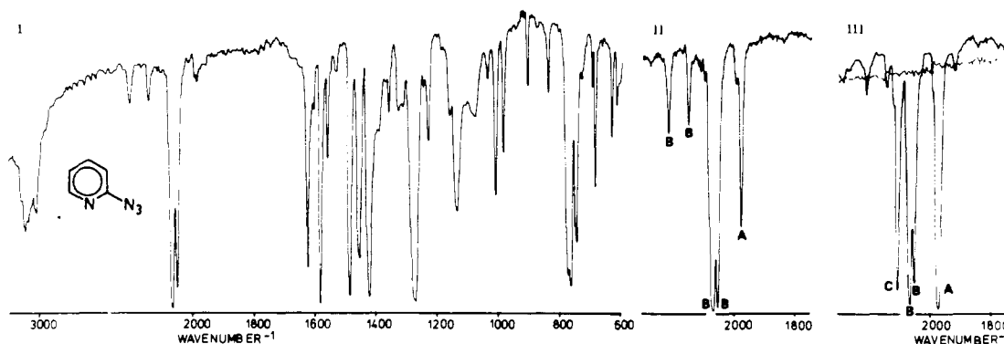
Figure 1. (I) Infrared spectrum of 2-pyridyl azide ( 9 ) at -196\text{ }^{\circ}\text{C} , obtained by pyrolysis of tetrazolo[1,5- a ]pyridine ( 8 ) at 200\text{ }^{\circ}\text{C} . (II and III) Partial infrared spectra ( -196\text{ }^{\circ}\text{C} ) of the pyrolysates of 8 at 370 and 480\text{ }^{\circ}\text{C} , respectively. The bands labeled A, B, and C are due to the carbodiimide 11 , the azide 9 , and 2-cyanopyrrole ( 12 ), respectively.
