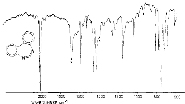
Figure 2. Infrared spectrum of dibenzo[ d,f ]-1,3-diazacyclohepta-1,2,4,6-tetraene at -196\text{ }^{\circ}\text{C} . Bands marked X are due to impurities.
